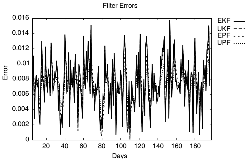
FIGURE 2.23 Filters Are Applied to the One-Dimensional Heston Model. The time series has a larger time-step \Delta t = 1.0 . Naturally, the errors are larger than the case where \Delta t = 1/252 .
