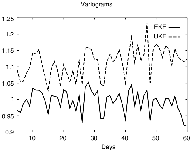
FIGURE 2.19 Variograms for Filtered Data via EKF and UKF. The input corresponds to a sequence of independent Gaussian random variables. As we can see, the variograms are close to one.
