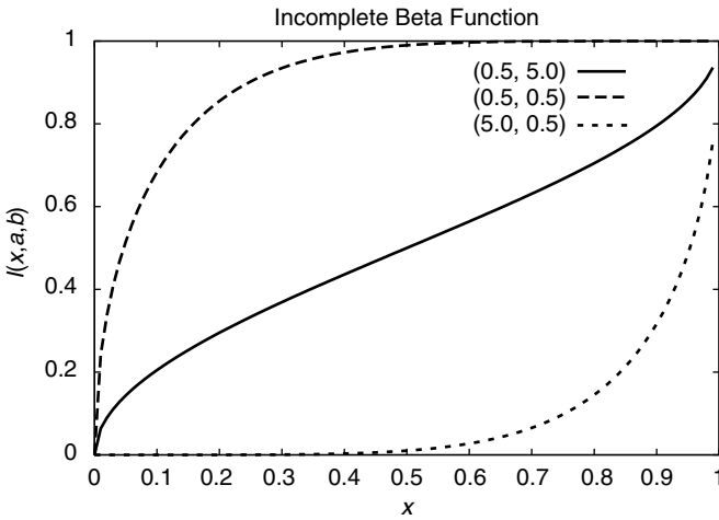
FIGURE 2.50 Plots of the Incomplete Beta Function. Implementation is based on code from Numerical Recipes in C .
